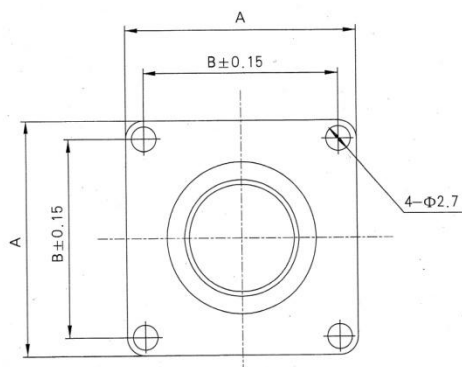
Square flange receptacle
